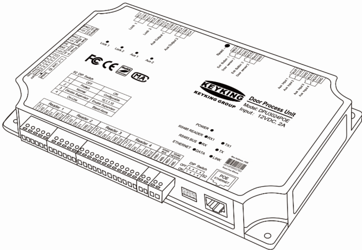
Figure 2-3-1 DPU3024POE controller
