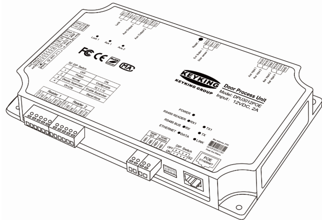
Figure 2-1-1 DPU3012POE controller
