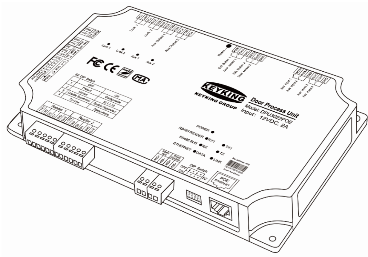
Figure 2-2-1 DPU3022POE controller
