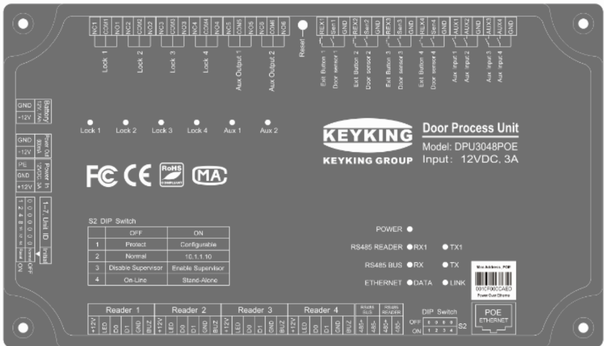
Figure 2-5-2 DPU3088POE wiring Schematic diagram
